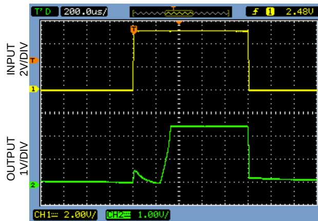
Power-On Transient Response
